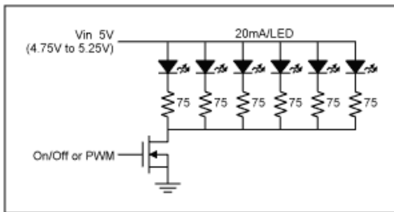
Figure 1. Most applications simply use a fixed bias voltage (5V in this case) and ballast resistors (75ohms in this case) to achieve approximate white LED brightness matching.
